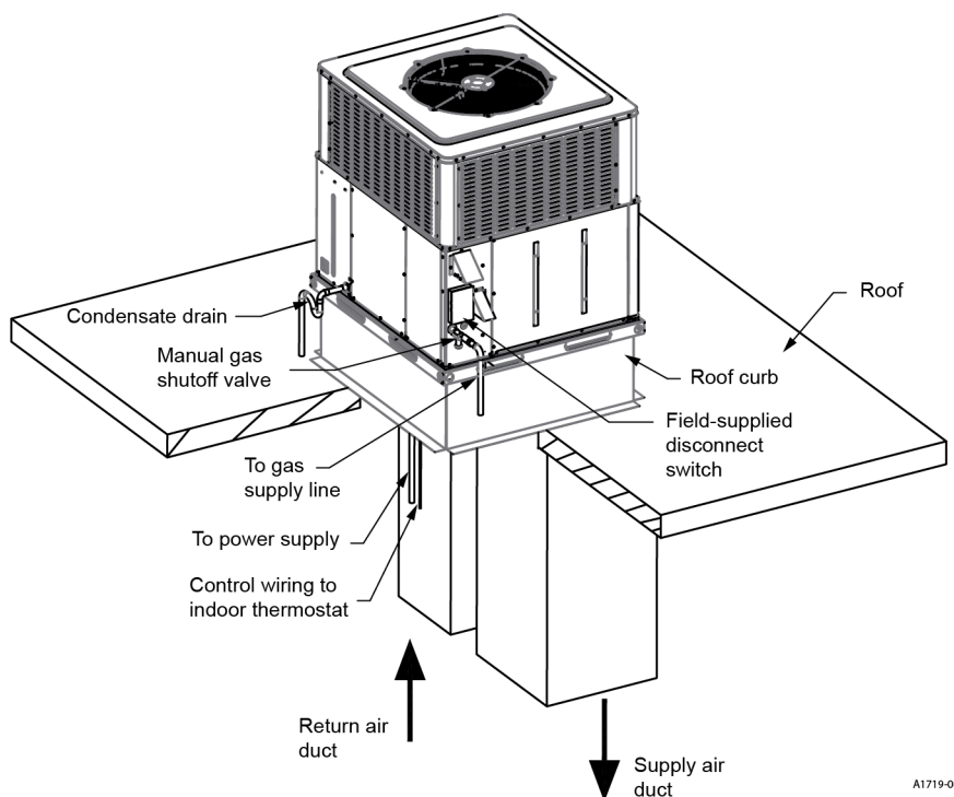
Figure 8: Typical installation on roof curb for unit
