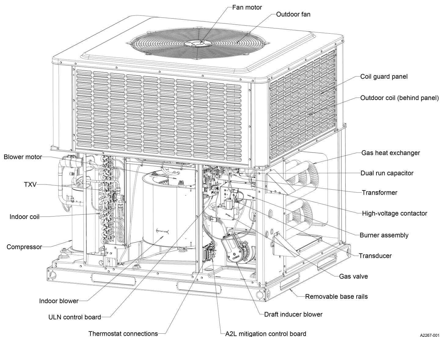
Figure 1: Unit components
