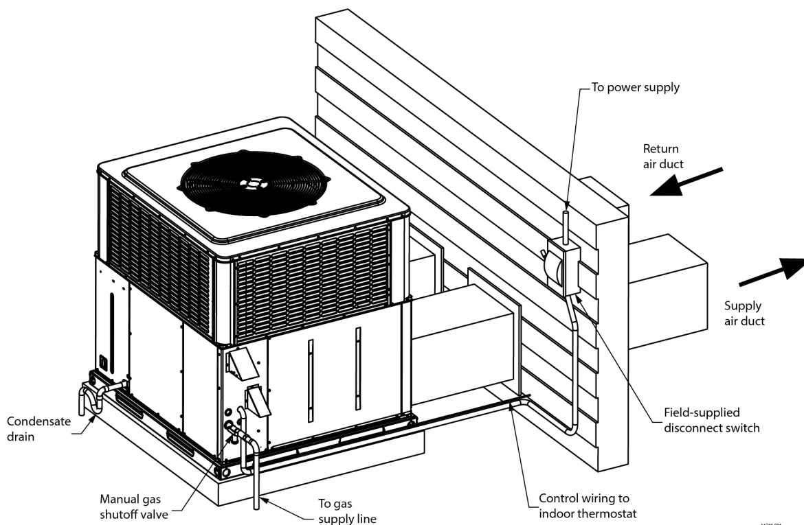
Figure 8: Typical ground installation on slab for unit
