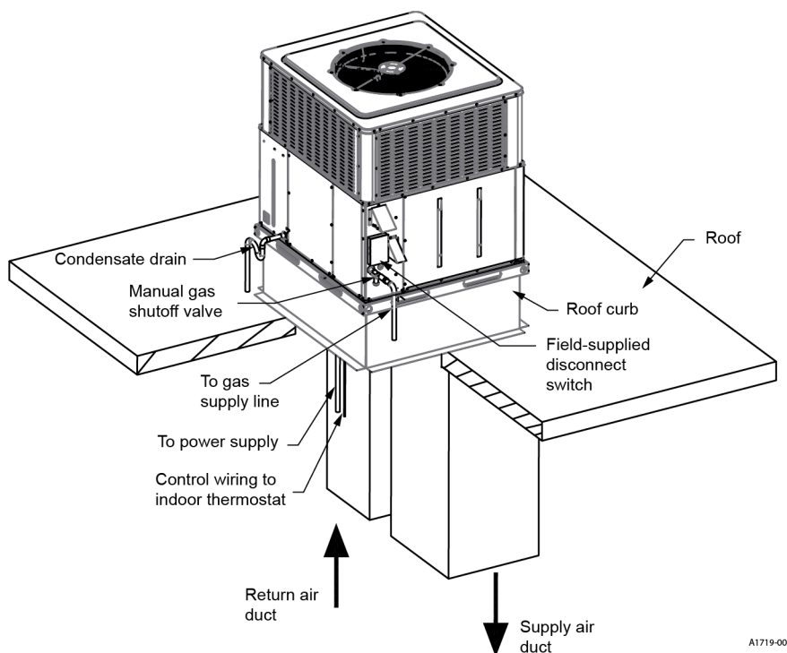
Figure 9: Typical installation on roof curb for unit
