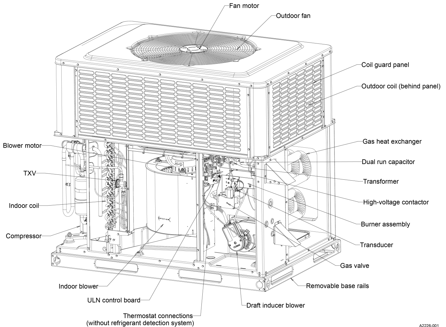
Figure 1: Unit components - PG3E24 and PG3E36 ULN units with rotary compressor
