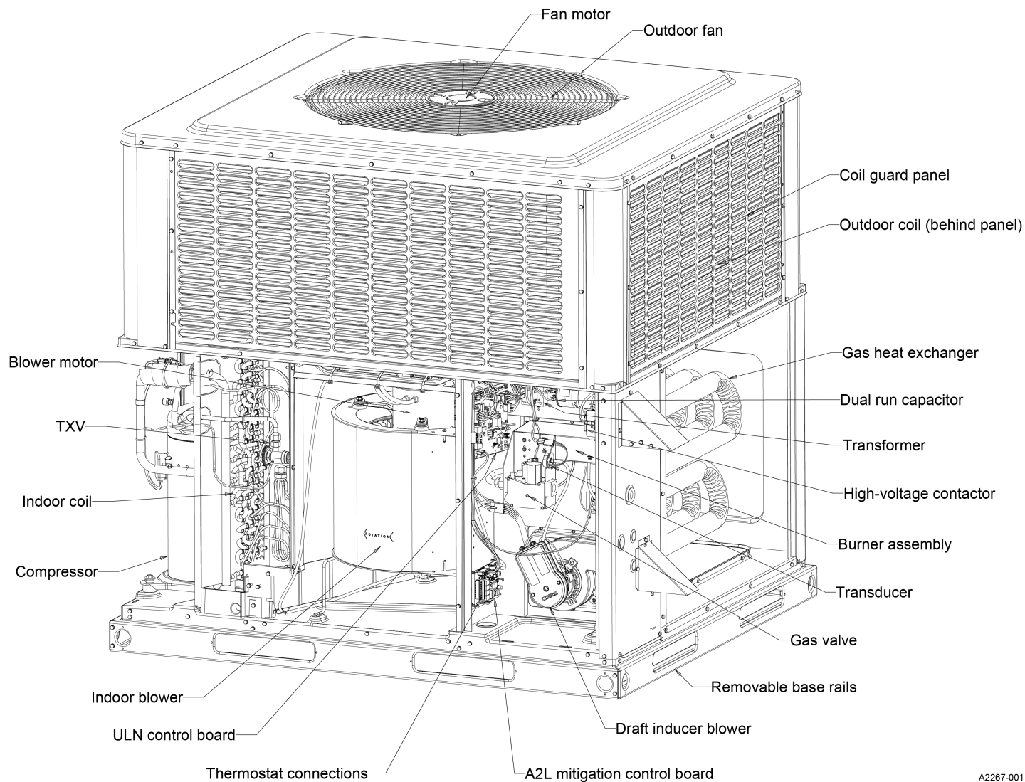
Figure 2: Unit components - PG3E48 and PG3E60 ULN units with scroll compressor and RDS
